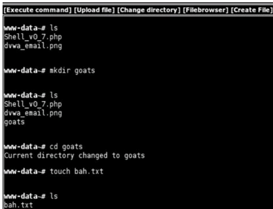
FIGURE 4.21 Executing custom commands on the DVWA web server via the web shell.
