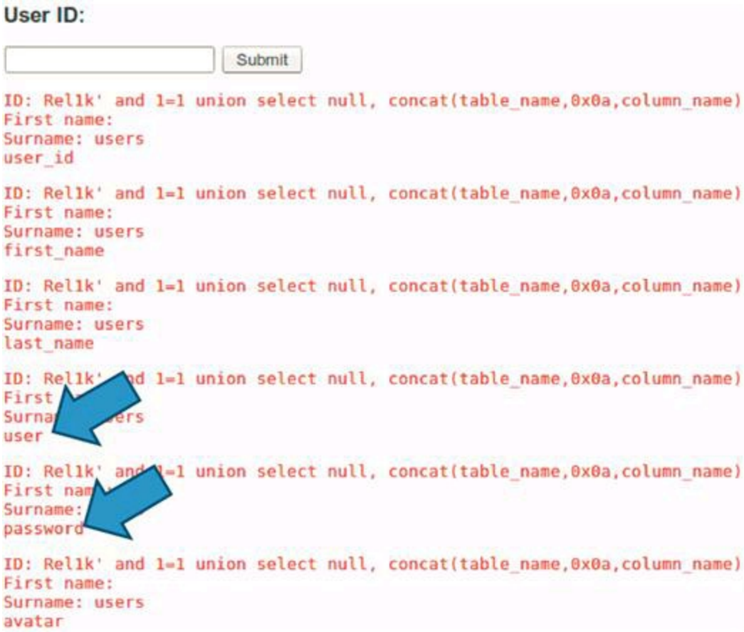
FIGURE 4.6 Results from injection accessing the information schema for the “users” table.
