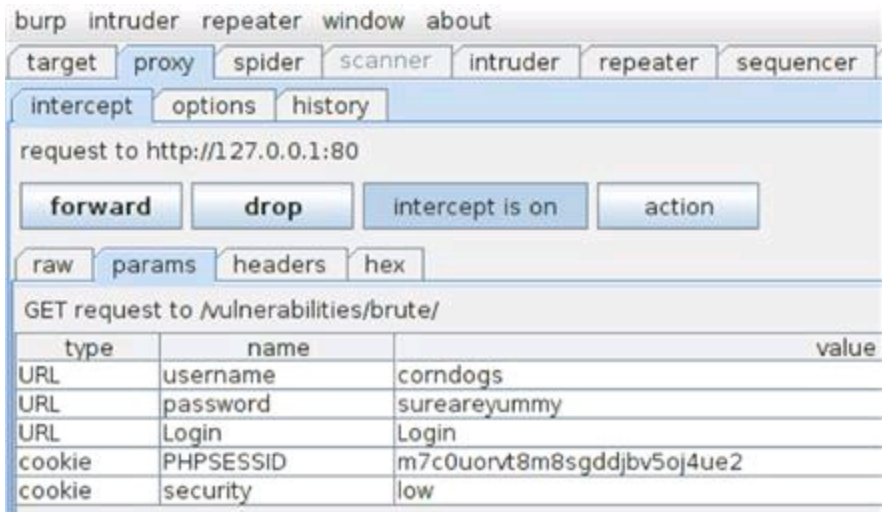
FIGURE 5.2 Intercepted authentication parameters in DVWA.
