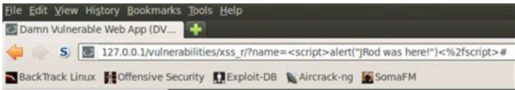
FIGURE 6.9 URL details of reflected XSS attack.
